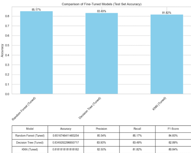
Figure 9: Comparison of Best three Models
