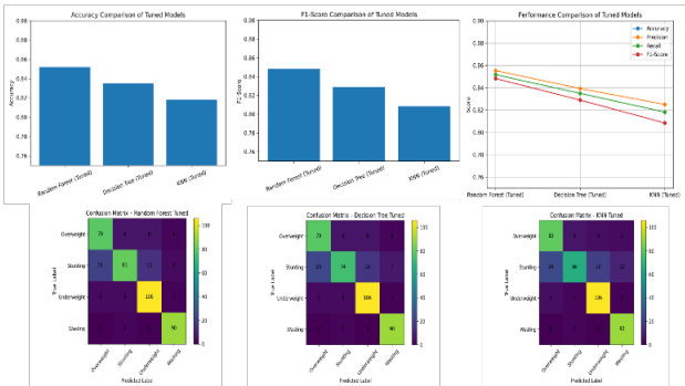
Figure 9: Comparison of best three Models
